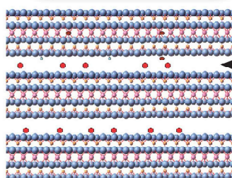
■ Typical montmorillonite (2:1 Phyllosilicate)
