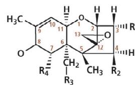
■ Type B-trichothecenes : DON (R1=OH, R2=H, R3=OH, R4=OH) NIV (R1=OH, R2=OH, R3=OH, R4=OH)
